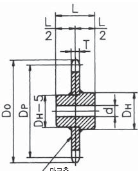
CW1형 CW1 TYPE
